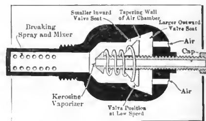
Fig. 2—Section showing principle of Speedo operation
